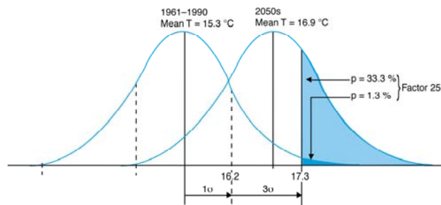
Figure 1: Effect of Change in Mean Temperatures on Extremes
