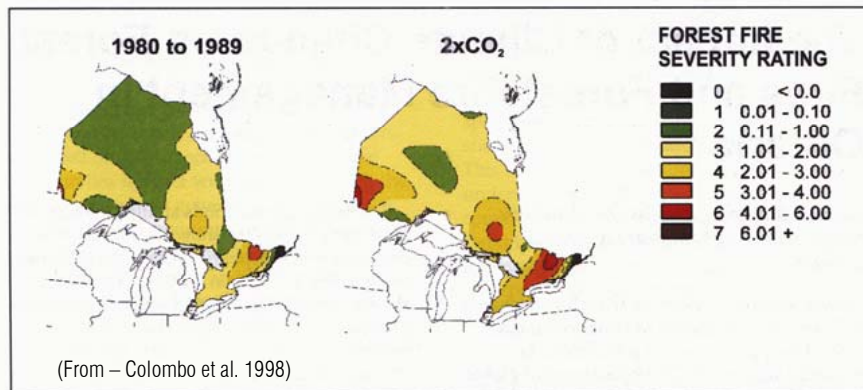
Figure 2: Change in Fire Disturbance Severity Rating for Ontario for a Doubled CO 2 Climate
