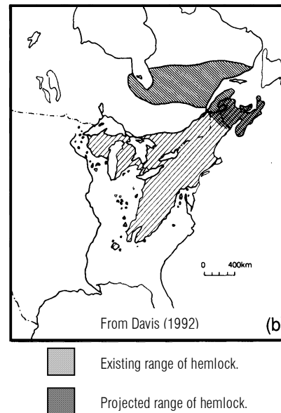
Figure 4: Impact of Climate Change on the Range of Eastern Hemlock (Davis, 1992)
