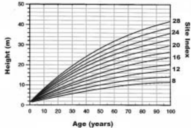
Figure 5: Site index curve for red pine
